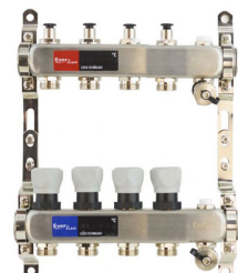
KIT DISTRIBUTOR CALORIFERE, 1"-3/4, 4 CAI, CU ROBINET TERMOSTATIC, ROBINET MICROMETRIC, AERISITOARE, ERMETIQ
