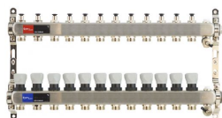
KIT DISTRIBUTOR CALORIFERE, 1"-3/4, 10 CAI, CU ROBINET TERMOSTATIC, ROBINET MICROMETRIC, AERISITOARE, ERMETIQ
